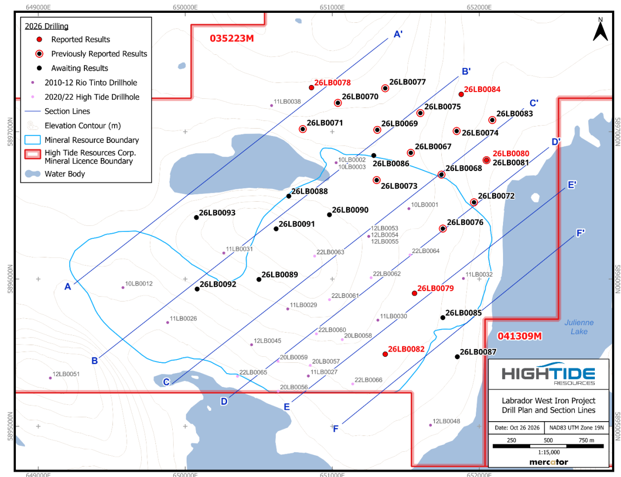
Figure 1. Labrador West Project – Plan map showing current mineral resource outline boundary, surface trace of vertical sections and location of drill holes.
