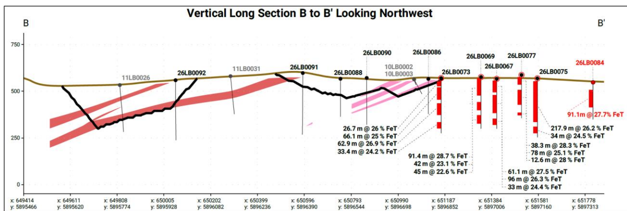
Figure 3. Labrador West Project – Long section B - B' - assays in red font are reported here and assays in black font have been previously reported.
